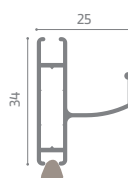
Handlebar
