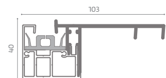
Recessed Profile
